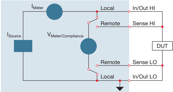
Source I, Measure V, I, or Ω configuration
