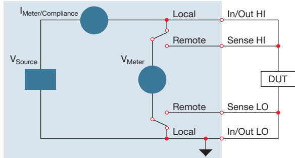
Source V, Measure I, V, or Ω configuration
